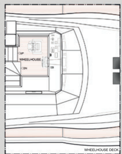
WHEELHOUSE DECK
